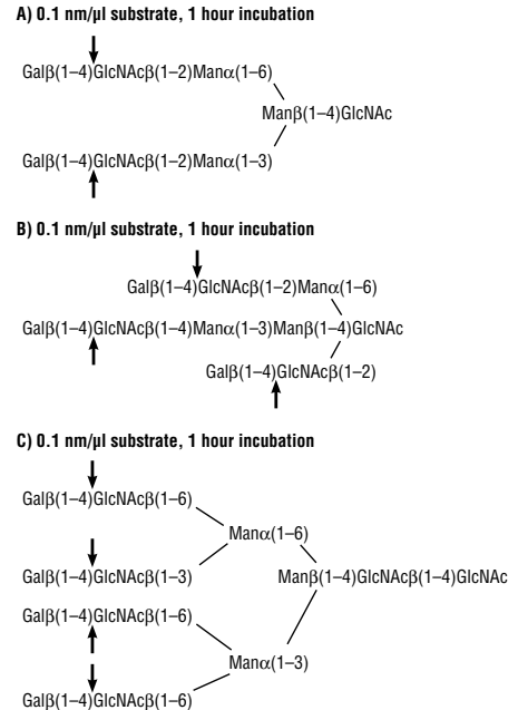
Figure 1: Detailed specificity of β1-4 Galactosidase. Reactions (A), (B) and (C) contained 2 units, 4 units and 8 units of β1-4 Galactosidase, respectively, and 1X GlycoBuffer 1 total reaction volume of 10 μl. Reactions were incubated at 37°C.
