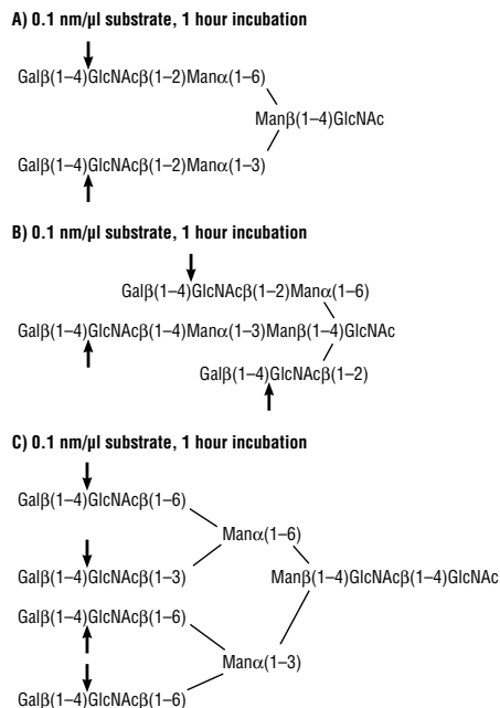
Figure 1: Detailed specificity of \beta 1-4 Galactosidase. Reactions (A), (B) and (C) contained 2 units, 4 units and 8 units of \beta 1-4 Galactosidase, respectively, and 1X GlycoBuffer 1 total reaction volume of 10 \mu l. Reactions were incubated at 37°C.
