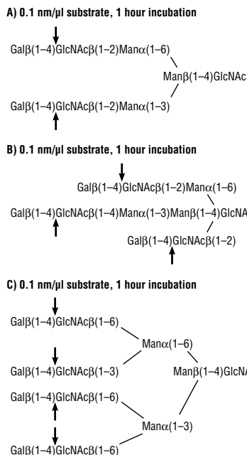
Figure 1: Detailed specificity of \beta 1-4 Galactosidase. Reactions (A), (B) and (C) contained 2 units, 4 units and 8 units of \beta 1-4 Galactosidase, respectively, and 1X GlycoBuffer 1 total reaction volume of 10 \mu l. Reactions were incubated at 37°C.
