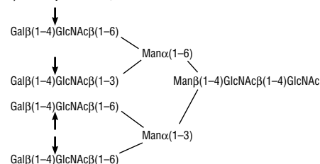
Figure 1: Detailed specificity of \beta 1-4 Galactosidase. Reactions (A), (B) and (C) contained 2 units, 4 units and 8 units of \beta 1-4 Galactosidase, respectively, and 1X GlycoBuffer 1 total reaction volume of 10 \mu l. Reactions were incubated at 37°C.
